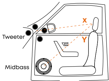
Installation example in a car
