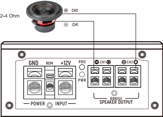
Bridged connection
