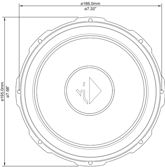
Speaker without adaptor ring
