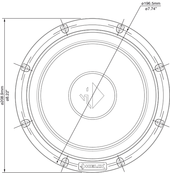
Woofer with assembled universal mounting ring
