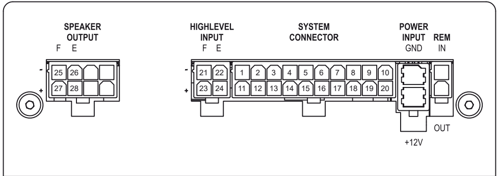
Fig. 1: Pin configuration UP 6DSP MK2
